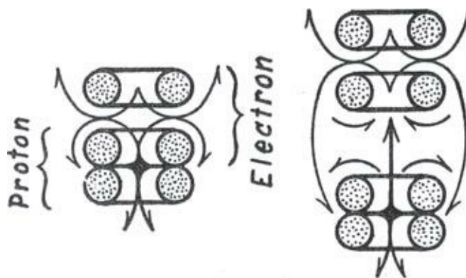
Krafft’s vortex Model of a Neutron(Left) and Hydrogen Atom (Right)
