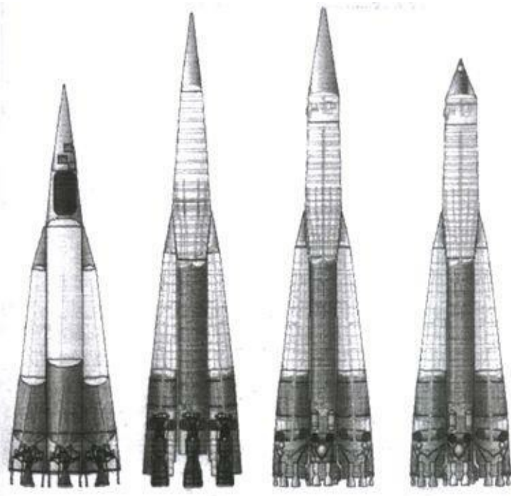
G-6 R-15 "Cluster of G-4's" 3000 kg fission warhead R-7 Initial Design RD-106/108 Engines 3000 kg fission warhead R-7 Final Design RD-107/108 Engines 5500 kg thermonuclear warhead R-7 / Sputnik 1 RD-107/108 Engines
